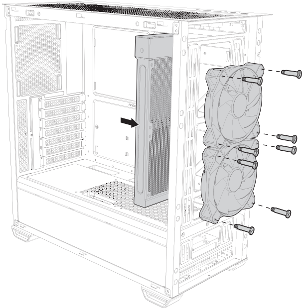
FRONT RADIATOR
