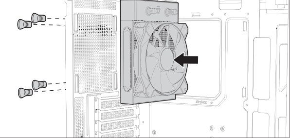
REAR RADIATOR
